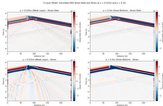
Figure: Horizontal Strain and strain rate for MPM-guided model. Plotted at crack depth (0.525) and at the snow bottom (0.3m). Gauge length is 10.4m.
